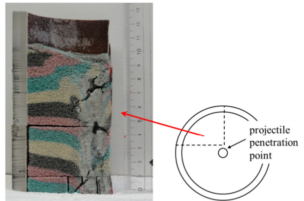
High pressure impact on geomaterials –grain crushing and structural evolution
